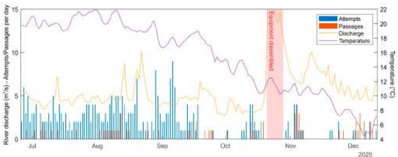
Figure 7. Upstream passage attempts per day and successful passages through the Palencia weir related to the river discharge and water temperature. The time-period with disassembled antennas (due to the damage risk by high flows) has been represented with a shaded area.
