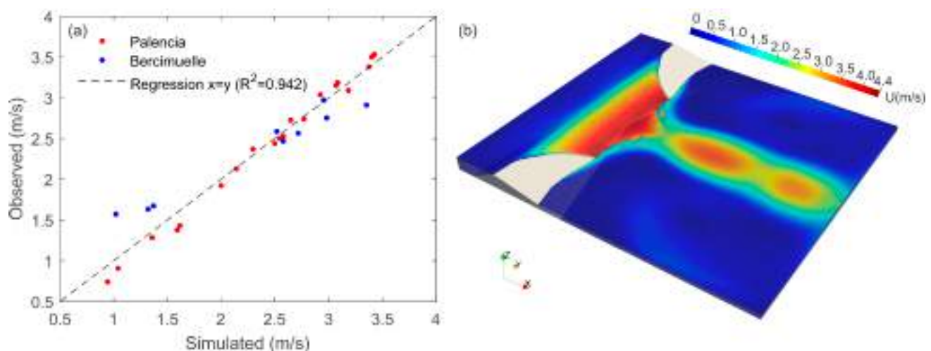
Figure 4. (a) Validation of the 3D model results considering field measurements ( R^2 stands for determination coefficient); (b) Simulation example of the flow velocity ( U ) for the Palencia weir ( p = 0.7 m, h_1 = 1.23 m; Q = 6 m 3 /s, d_2 = 0.46 m).
