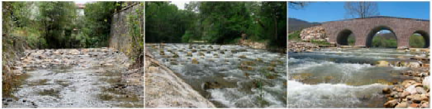
Figure 2. Left: bottom semi-dry bottom ramp [R- bt-sd ] in Azkoitia (Gipuzkoa). Center: boulder ramp [R- bl-c ] in the Najerilla River, La Rioja. Right: concrete pool-and-weir ramp [R- pw-c ] in the Pisuega River, northern Palencia. All of them are full-width NLFs—the device extends across the entire width of the river channel, from one bank to the other—and the structures are positioned downstream relative to the barrier.
