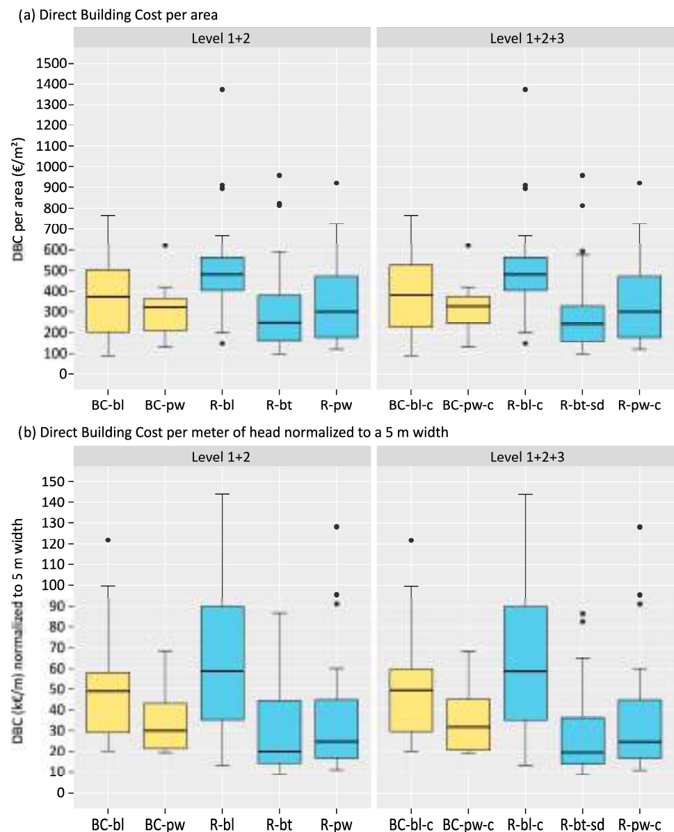
Figure 7. Box-plots for construction costs (a) per area (€/m 2 ) and costs (b) per height for a width of 5 m (€/m) for each type of solution (level 1 + 2 and level 1 + 2 + 3). Categories “BC-bl-d”, “BC-pw-d” and “R-bt-c” are not included because they contain only a single data point. The centerline corresponds to the median and dots represent the outliers.
