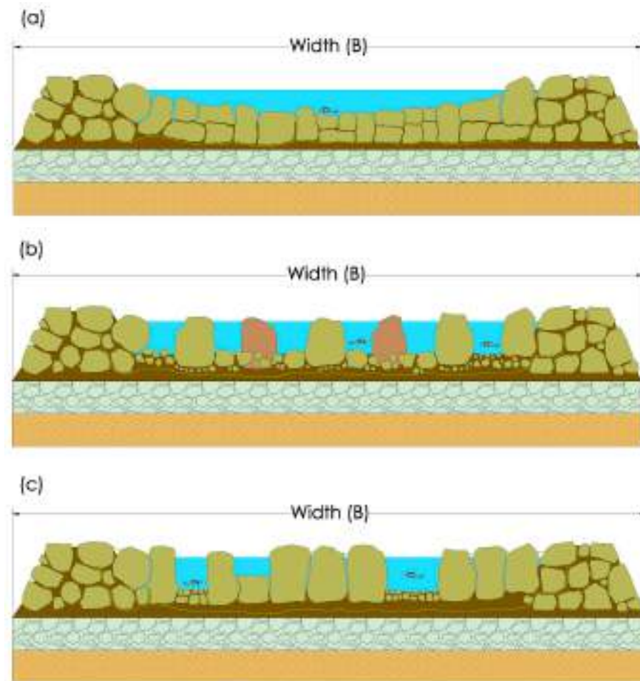
Figure 3. (a) Cross-section of a semi-dry bottom ramp [R-bt-sd]; (b) cross-section of a boulder ramp with concrete slab and sidewalls [R-bl-c]; (c) cross-section of a pool-and-weir system with concrete [R-pw-c].
