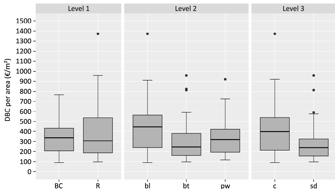
Figure 6. Box-plots for construction costs per area (€/m 2 ) by levels. 1: ramp (R), bypass channel (BC); 2: boulder type (bl), bottom type (bt), pool-and-weir system (pw); 3: concrete structures (c), semi-dry structures (sd). Category “dry structures” (d) is not included because it contains only a single data point. The centerline corresponds to the median and dots represent the outliers.
