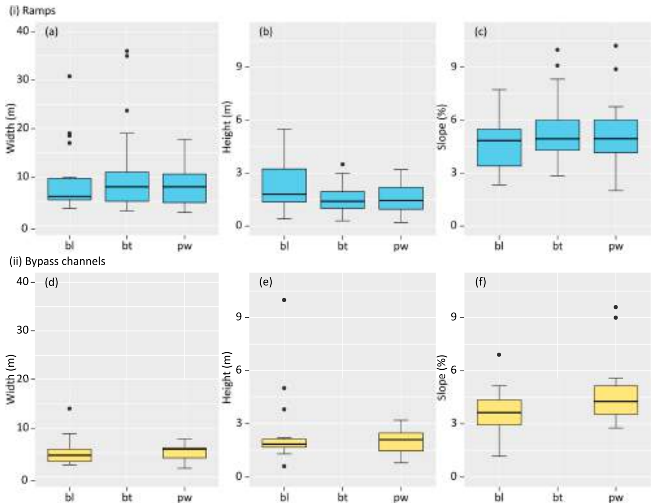
Figure 5. Box-plots for width, height, and slope by construction type: bl (boulder), bt (roughness bottom), and pw (pool-and-weir) for ramps (a–c) and bypass channels (d–f). The centerline corresponds to the median and dots represent the outliers.
