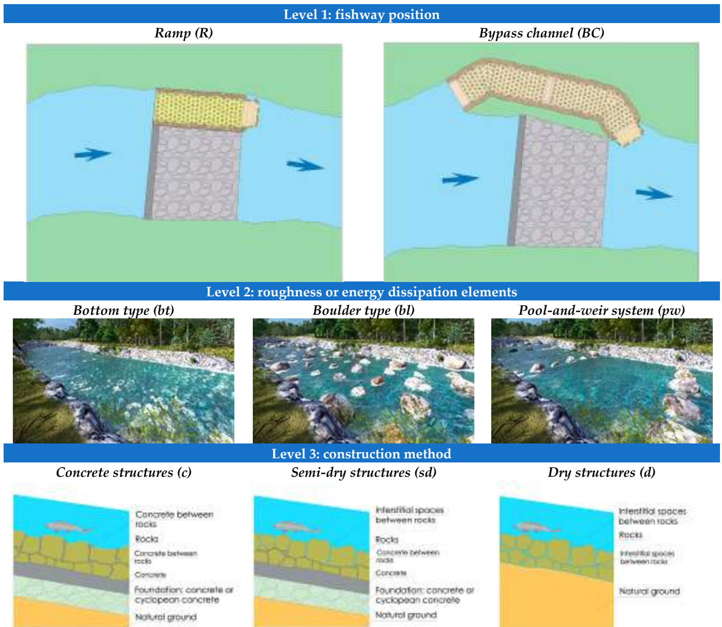
Figure 1. Classification of nature-like fishways according to the three hierarchical levels considered in this study.
