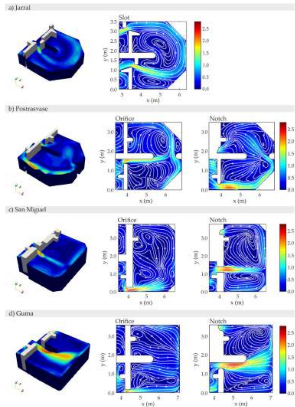
Figure A1. u (m/s) turning pool contours in the middle section of the orifice, notch, and slot.
