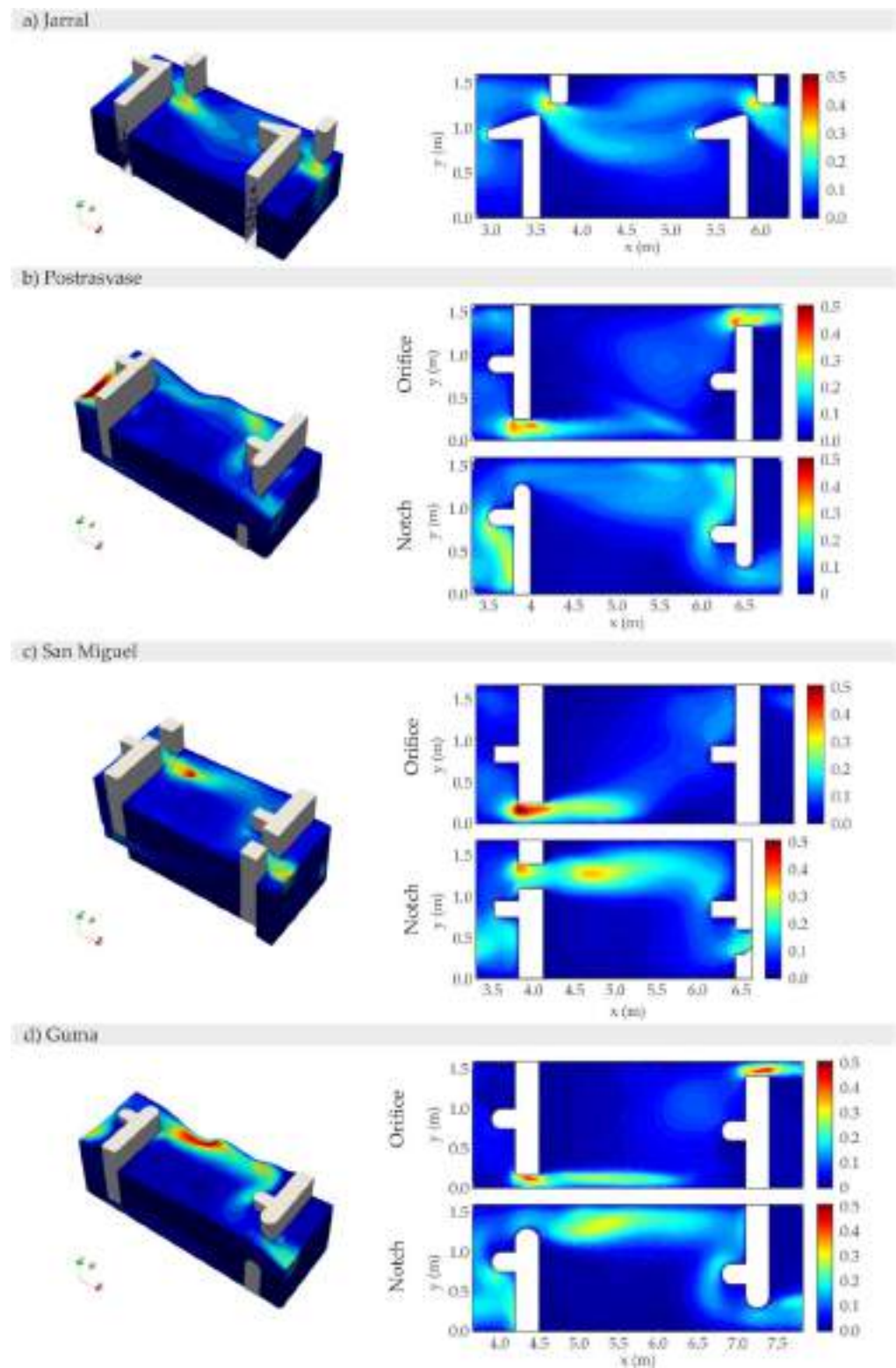
Figure A4. k (J/kg) straight section contours in the middle section of the orifice, notch, and slot. Appendix A.3. Vorticity Contours
