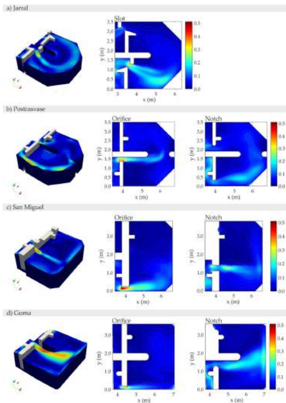
Figure A3. k (J/kg) turning pool contours in the middle section of the orifice, notch, and slot.
