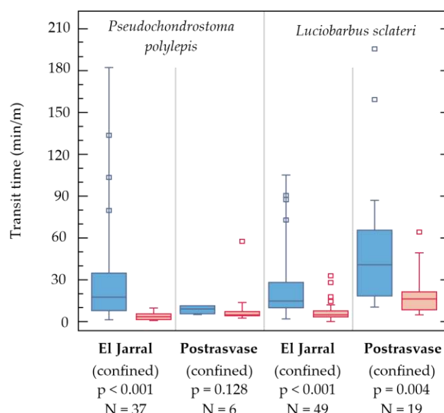
Figure 5. Box-plot distribution of transit time (standardized to minutes per meter of height ascended) for turning pools (blue box) and straight sections (red box), separately by species (left: P. polylepis ; right: L. sclateri ). p -value refers to the comparison of median values between turning and straight sections of the same field test case. N = number of events.
